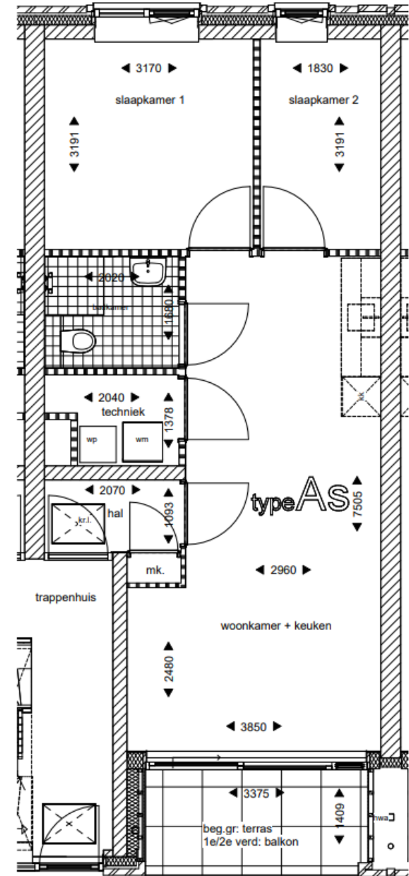
Appartement type As (gespiegeld)
